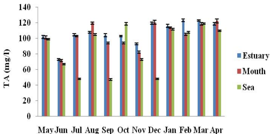
Fig.10.Monthly variation of Total alkalinity vellar estuary, mouth and coastal waters of Parangipettai during May 2011-April 2012
