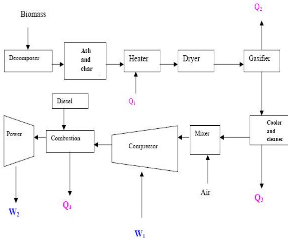
Figure 7 Advanced biomass power with diesel engine (Omer, 2006).
