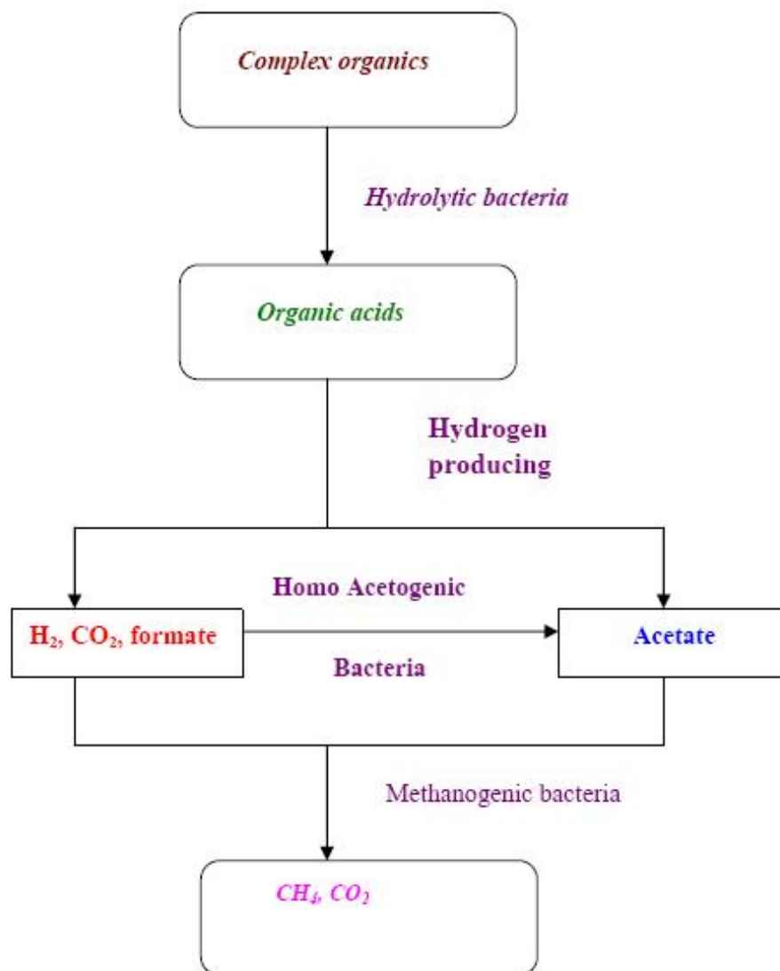
Figure 3 Biogas production process (Omer, 2003).
