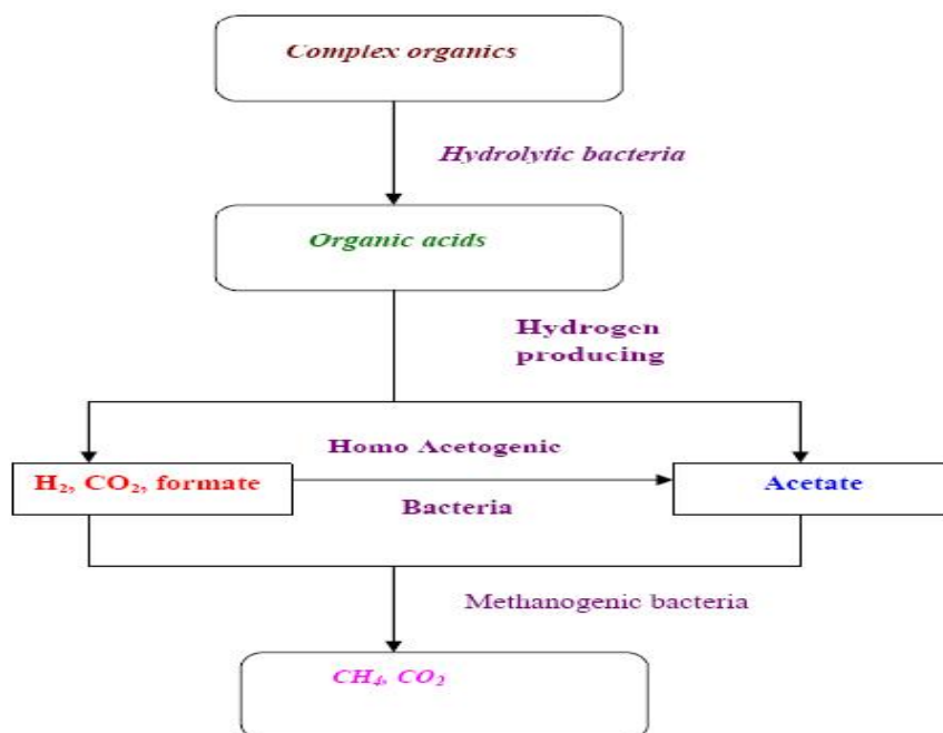
Figure 3. Biogas production process (Omer, 2003).
