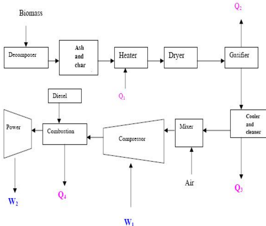
Figure 7. Advanced biomass power with diesel engine (Omer, 2006).
